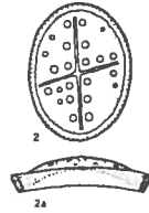
FIGS. 2, 2a — Arkhangelskiella obliqua n. sp., 2) plan view, 2a) side view; x 4000.
