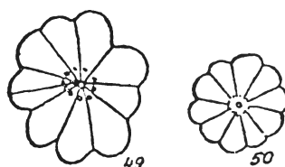
Figs. 49-50 — Discoaster olteniae n. sp.
